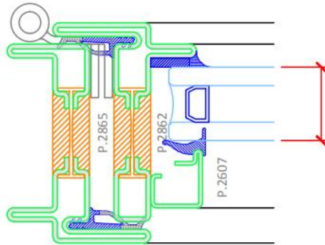
Outward Opening Window
