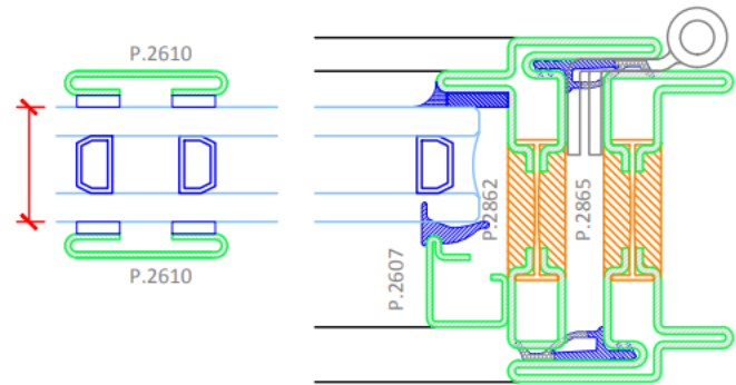
Outward Opening Door
