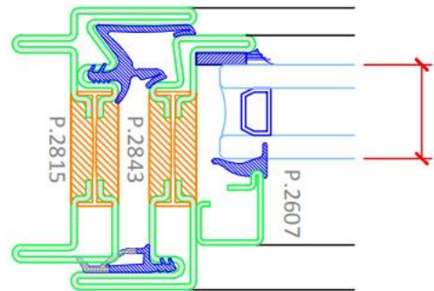
Horizontal Pivot Window- Top
