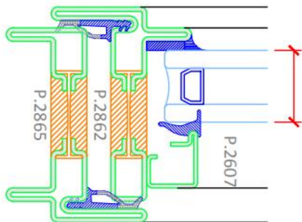
Horizontal Pivot Window- Bottom
