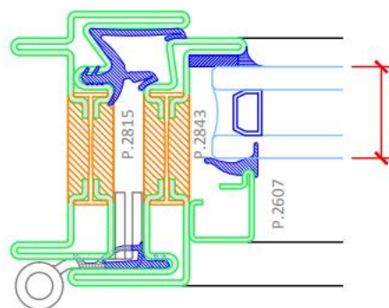
Inward Opening Window
