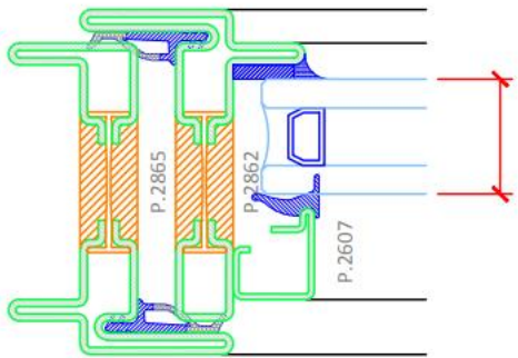
Outward Awning Window
