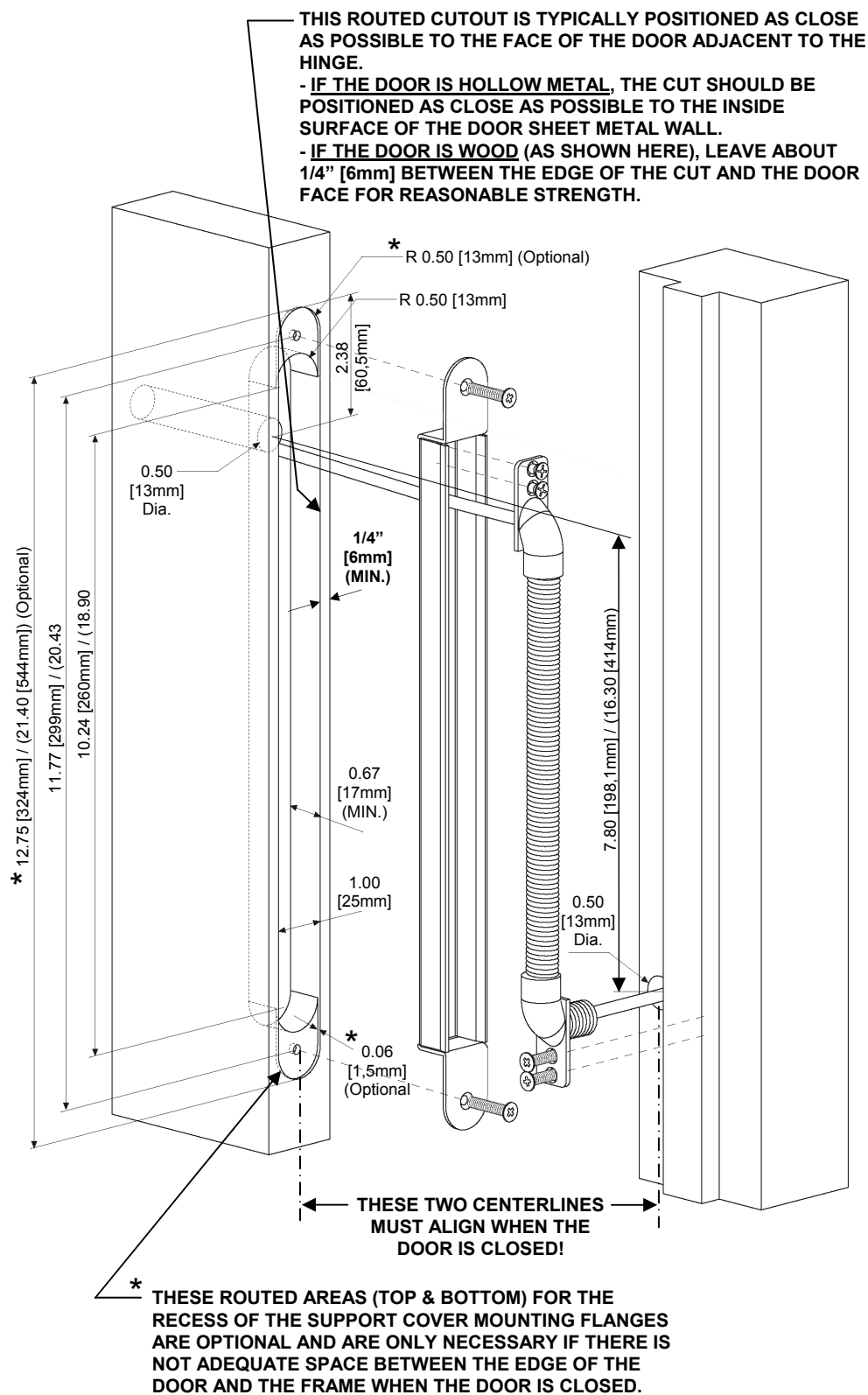
Figure 3: ROUTING DETAIL
